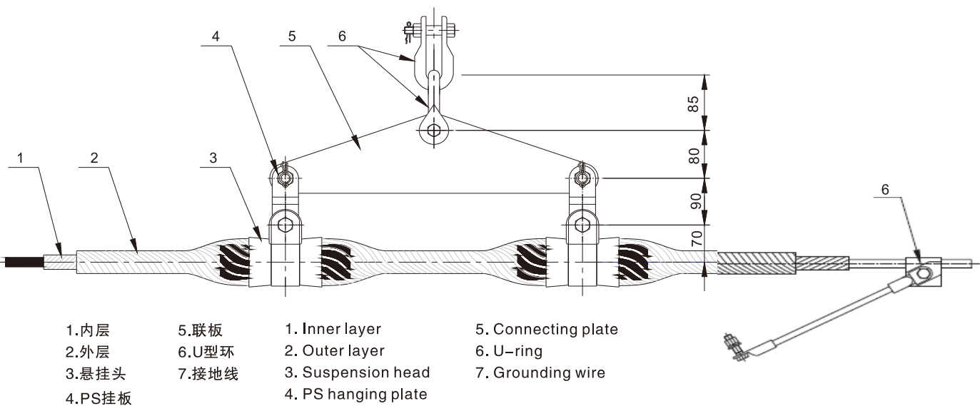
双悬垂线夹 (表8.3) Double suspension clamp (Table 8.3)
