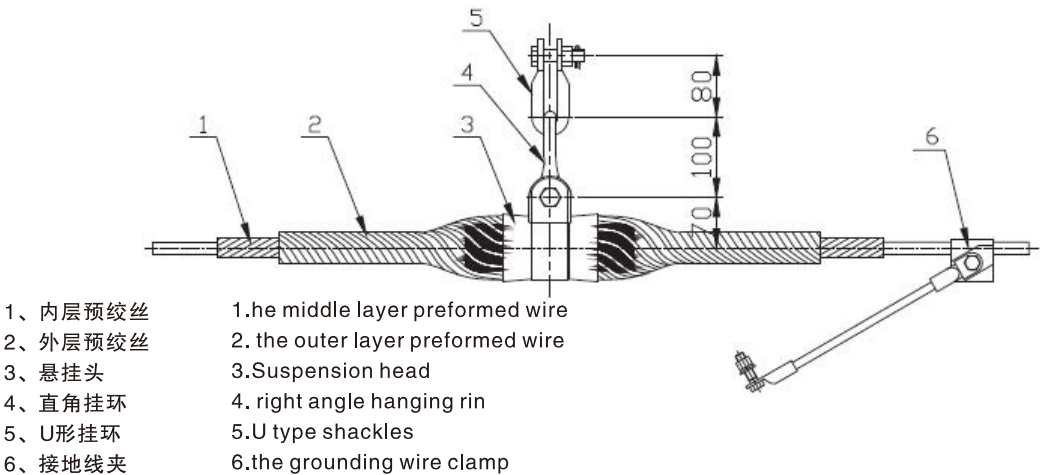
单悬垂线夹(表8.2) Single suspension clamp (Table 8.2)
