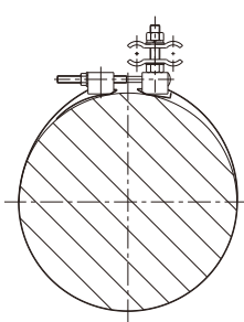
金属型杆用引下夹具 Metal type rod for lowering fixture
