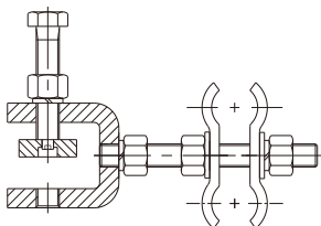
金属型塔用引下夹具 Metal type tower lowering fixture
