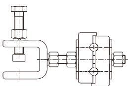
橡胶型塔用引下夹具 Rubber type tower lowering fixture
