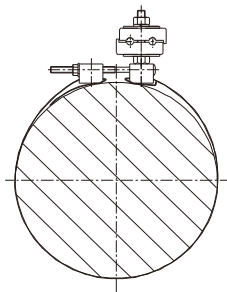
橡胶型杆用引下夹具 Rubber type rod for lowering fixture
